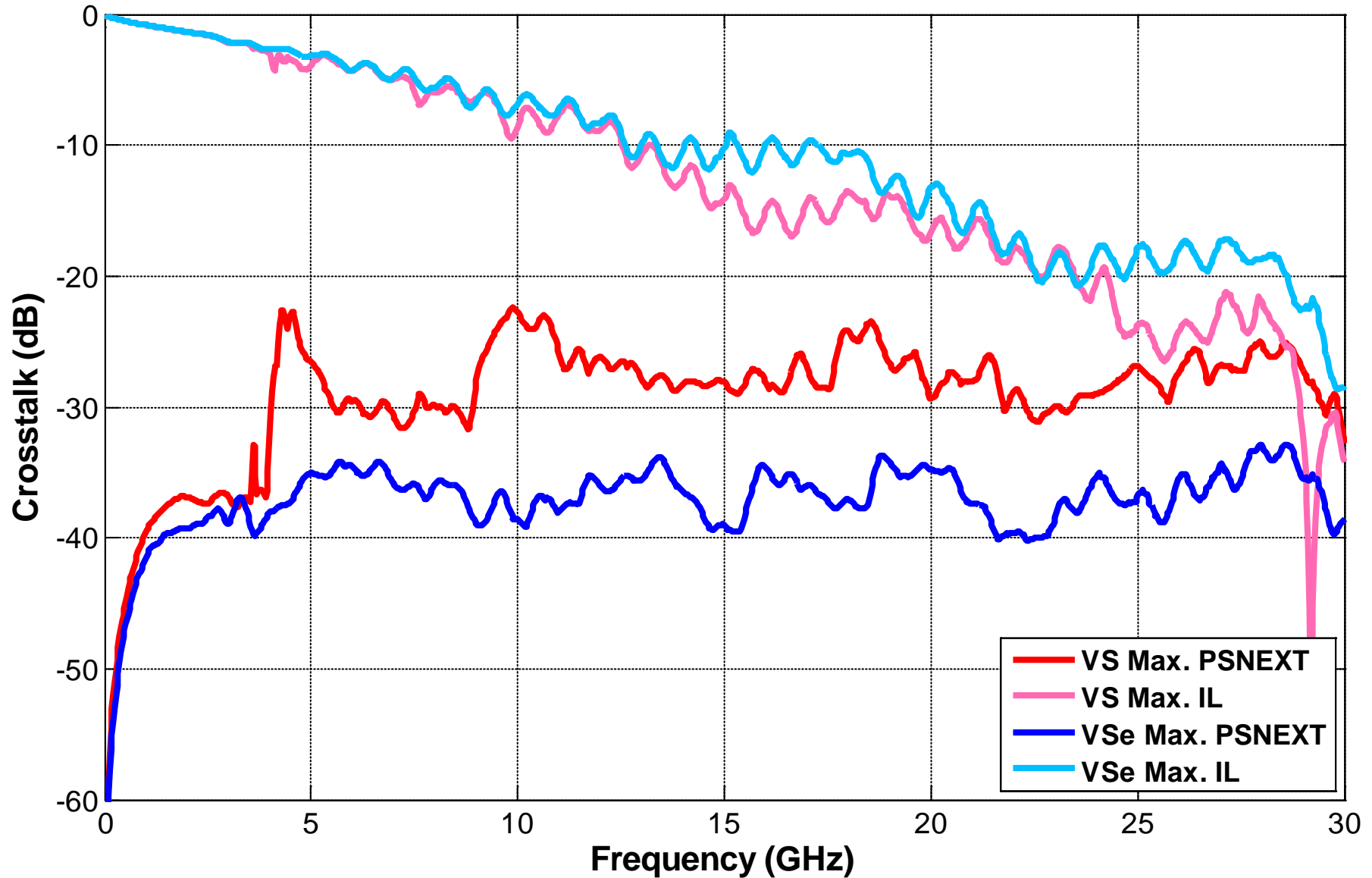
AirMax VS vs VSe Maximum Power-Summed NEXT
