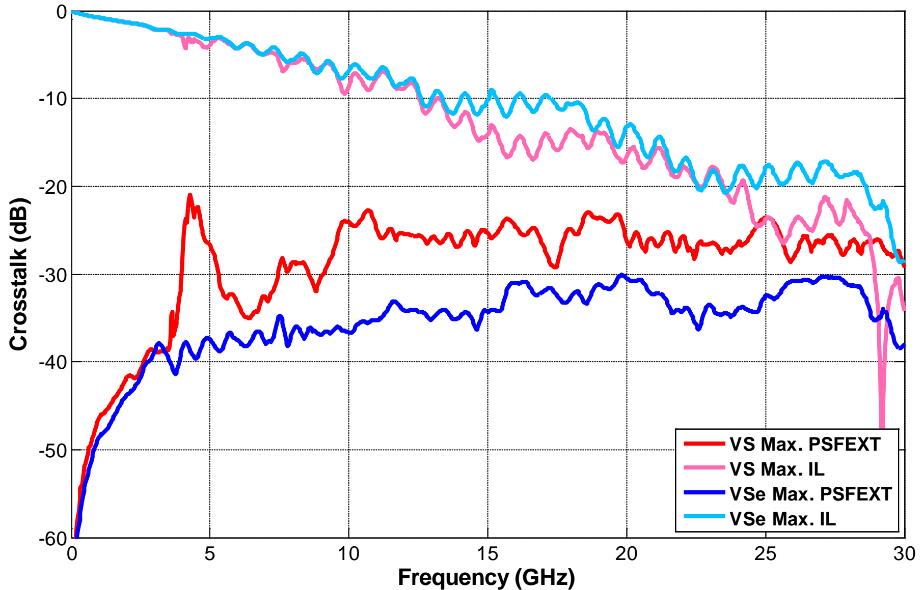
AirMax VS vs VSe Maximum Power-Summed FEXT
