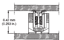
SURFACE-MOUNT RECEPTACLE TO 6.74 mm (0.226 in.) TALL SURFACE-MOUNT HEADER
