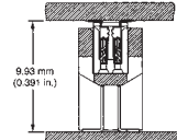
SURFACE-MOUNT RECEPTACLE TO 9.25 mm (0.364 in.) TALL SURFACE-MOUNT HEADER
